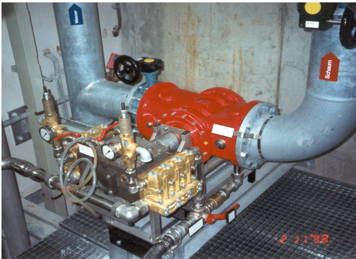
FireDos FD6000/3-PP-S
